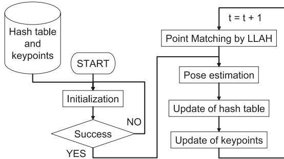
Figure 4: Process flow. On-line update of keypoints and the hash table starts after the initialization is finished.
