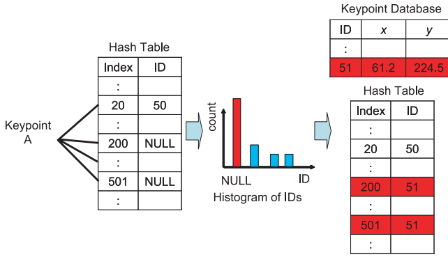
Figure 3: On-line update of new discriminative keypoints. Since keypoint A is new based on the number of NULL, new ID (No.51) and its xy are stored in the database. Also, No.51 is inserted at the indices of NULL.
